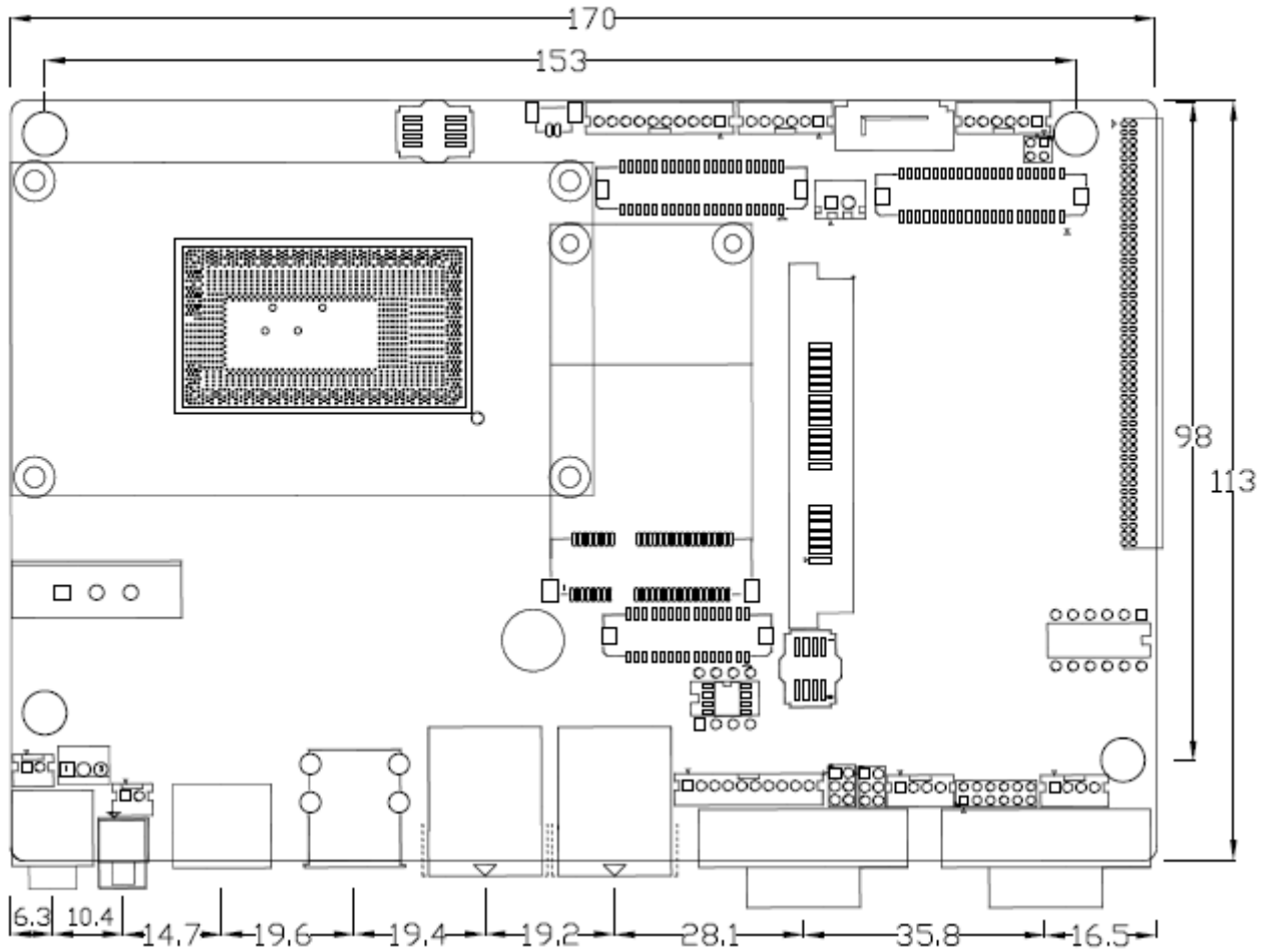
Figure 2.1: Motherboard Dimensions
